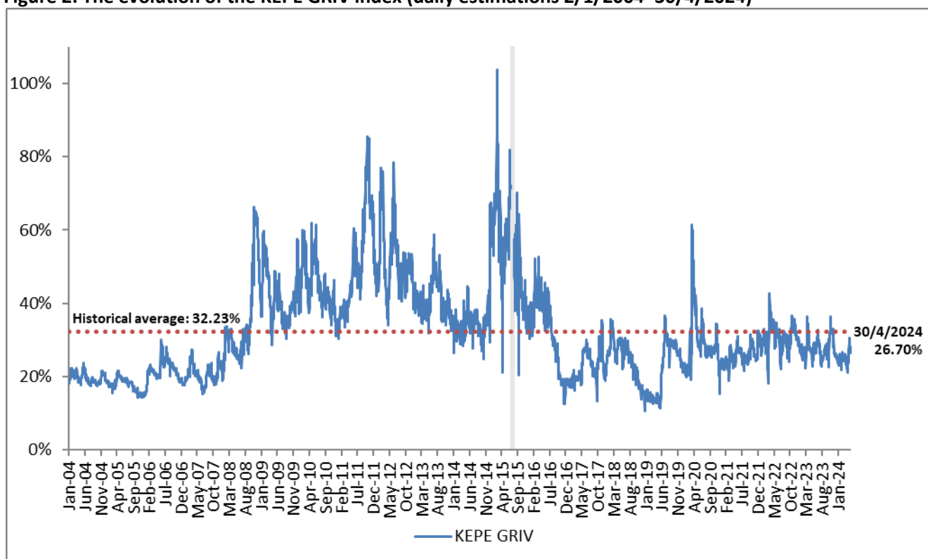
Figure 2: The evolution of the KEPE GRIV index (daily estimations 2/1/2004–30/4/2024)
